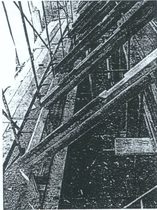
Figure 4 The rafters of the Fig House in the Holkham kitchen gardens. The 1872 timbers have benefited from the application of warm raw linseed oil. Note the lightness of the as-yet-untreated timbers and the relative lack of new wood required in these repairs, undertaken during 2001.
